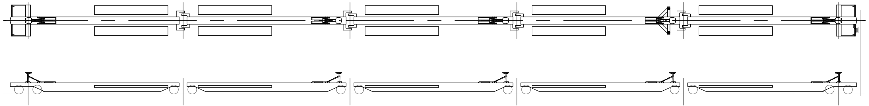
Flat Car: Articulated Spine Car-TOFC
